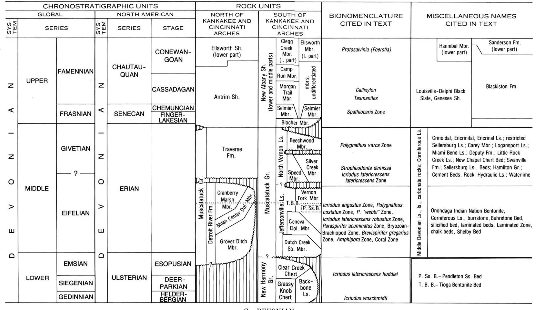
C. DEVONIAN
