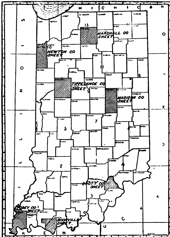
FIG. 1.—Sketch map showing location of the Tippecanoe County area, Indiana.
